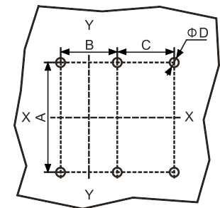
Front connection(mm)
