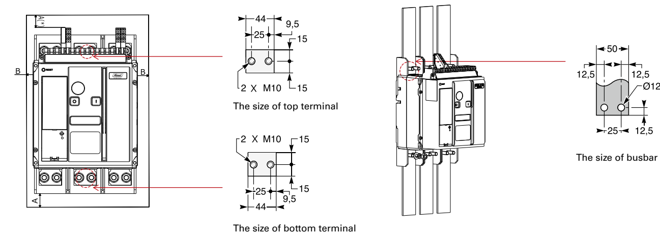
Terminal and busbar dimensions (mm)
