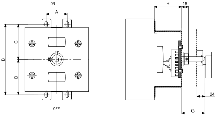
Handle and door cutting dimensions(mm)
