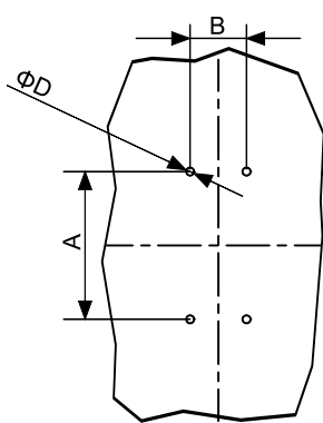
Front connection (mm)
