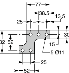
Extension terminal for N phase or C phase of 4 pole
