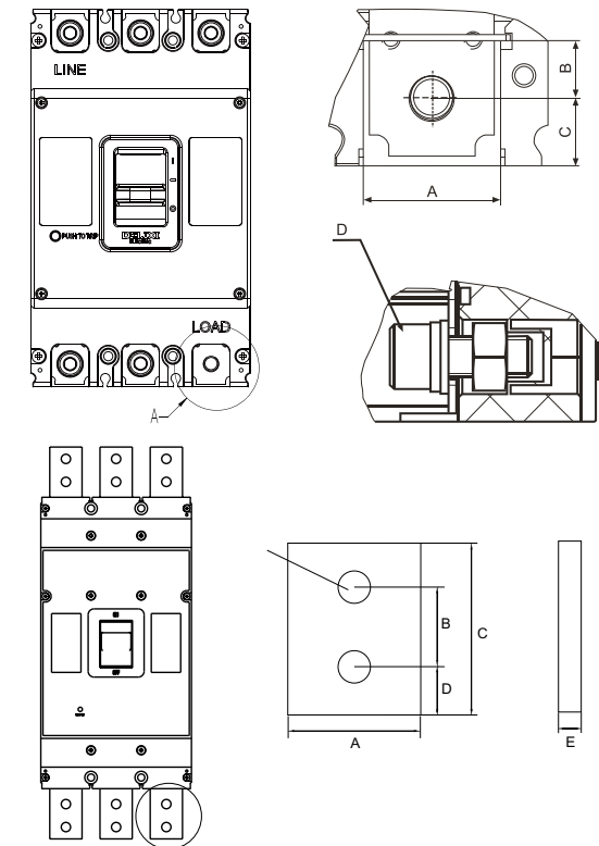
Connecting conductor (mm 2 )
