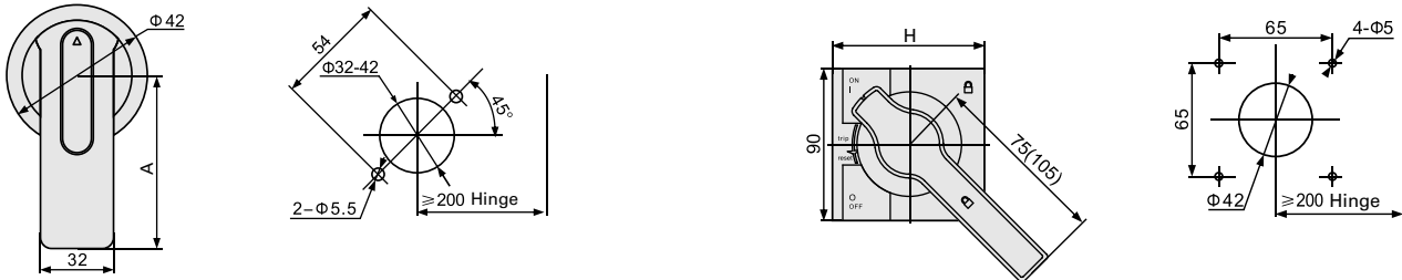
Round handle dimensions
