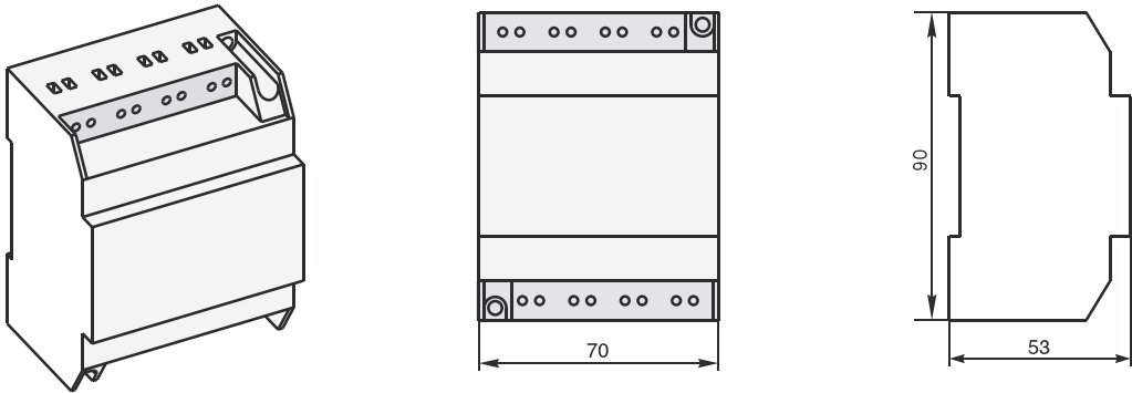
Dimensions of power module (35mm Dim rail fitted)
