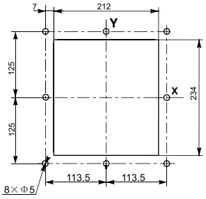
With doorframe: Holes dimension on door
