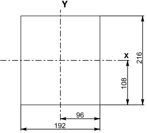
Without doorframe: Holes dimension on door
