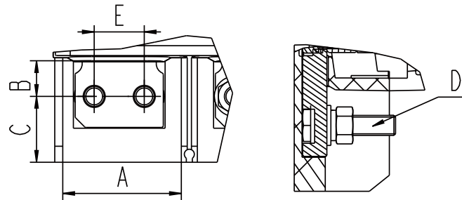
Terminal connection dimensions (mm)
