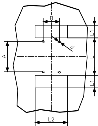
Rear connection(mm)
