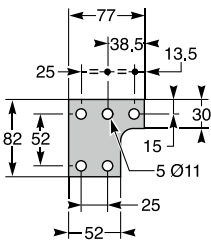
Extension terminal for A phase or B phase of 4 pole
