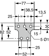
Extension terminal for B phase of 3 pole
