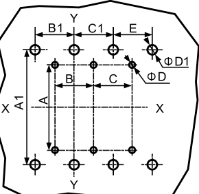
Rear connection(mm)
