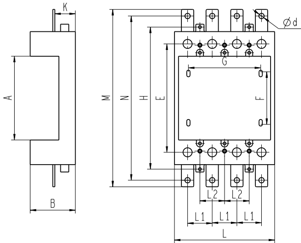
Plug-in front hot position drawing
