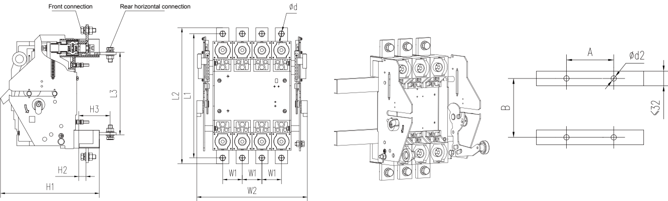
Rear connection(mm)
