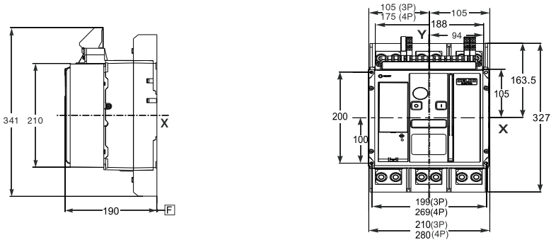
Fixed MCCB mounting dimension (mm)
