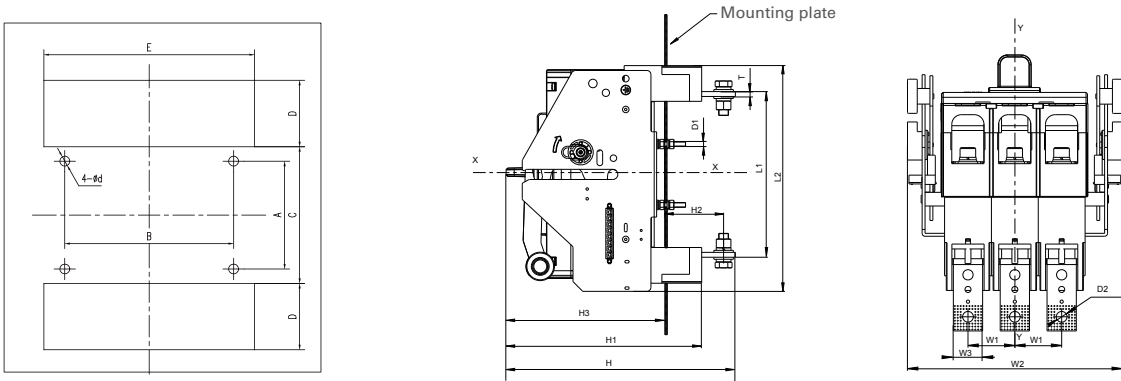
Rear connection(mm)
