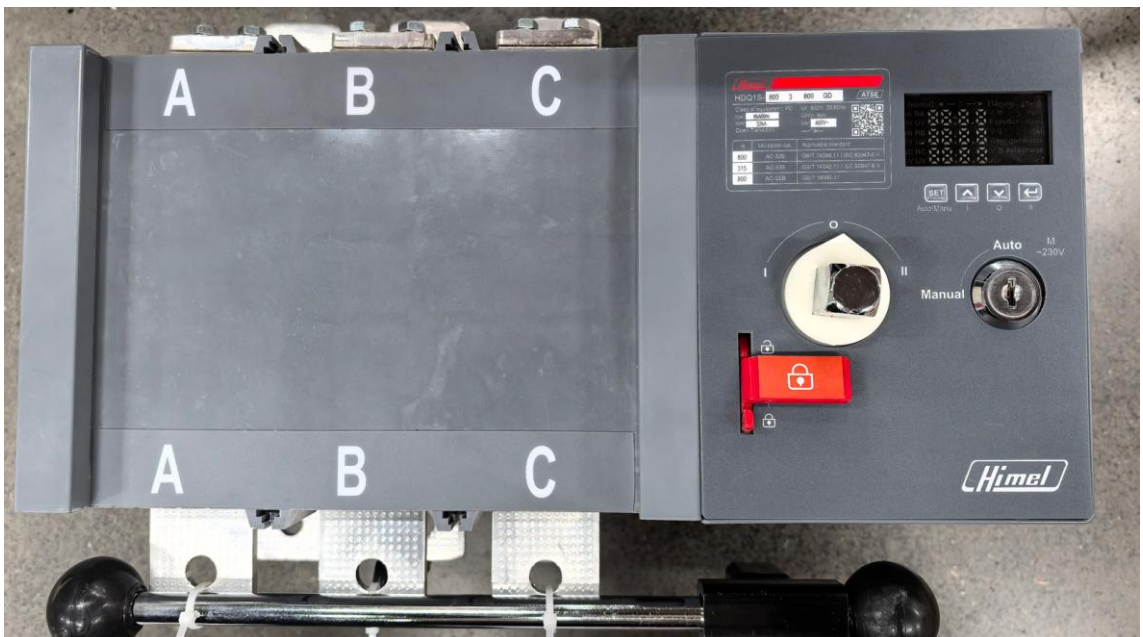
Outer construction of HDQ1S-800380GD
