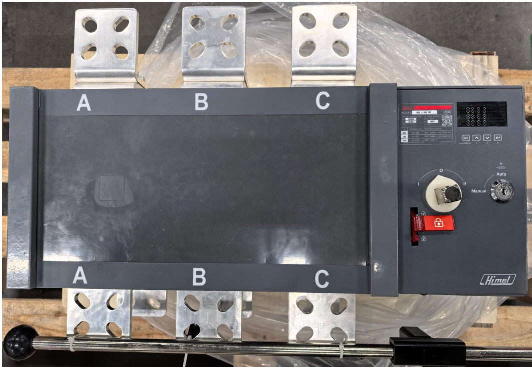
Outer consturction of HDQ1S-160030800GD
