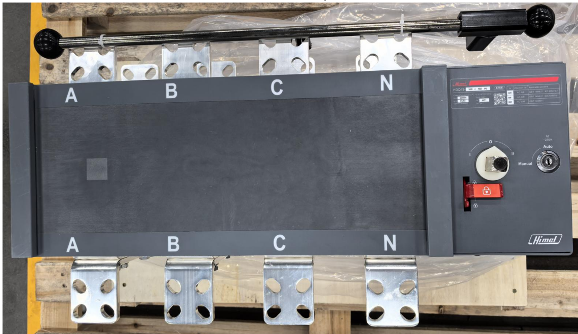
Outer consturction of HDQ1S-160041600PU
