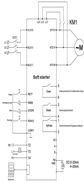
Wiring diagram
