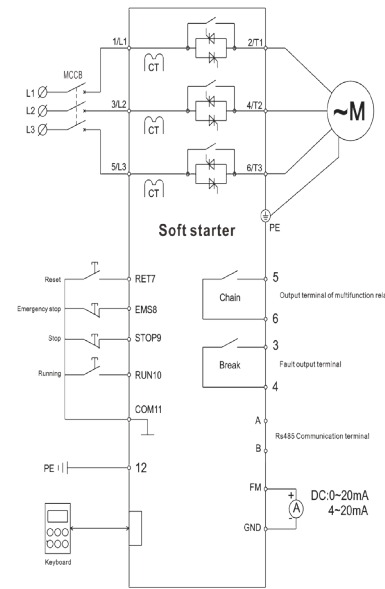
Wiring diagram
