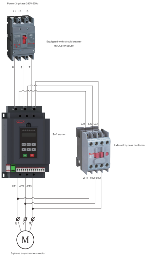
Connection diagram
